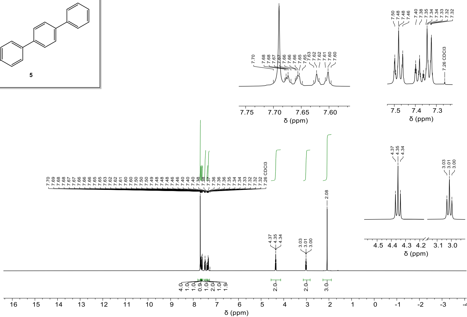
1 H NMR (400 MHz, CDCl 3 ) of [4-(4-phenylphenyl)phenyl] ethyl acetate (5).
